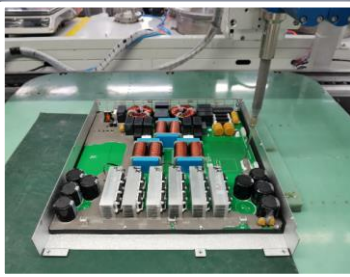
Single Board Assembly
